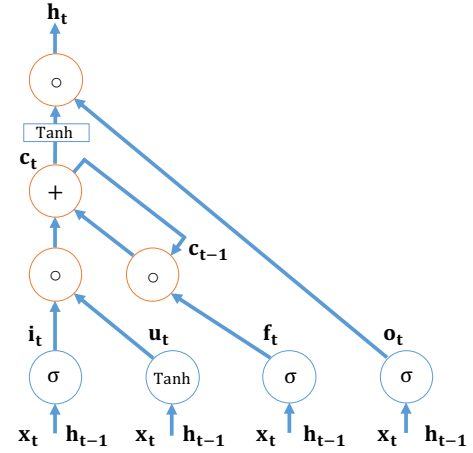
Fig. 2. The structure of a LSTM layer. The input \mathbf{x}_t of the first layer is the geometric feature. For higher layers, the input \mathbf{x}_t is the output \mathbf{h}_t from the previous layer at the same time instance.
