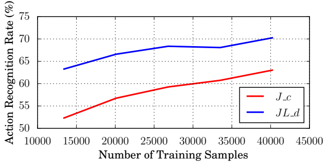
Fig. 15. Influence of training data samples. The performance of the LSTM model using JL_d decreases slower than using J_c , with decreasing training samples.
