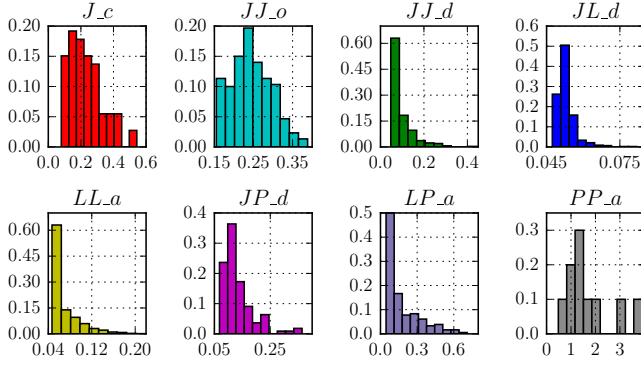
Fig. 11. The histogram of s_i calculated by Eqn. (8). x axis represents the value of s_i and y axis represents the percentage of s_i with the same value.
