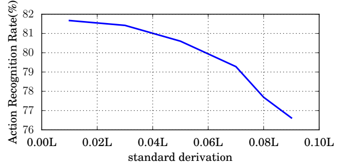
Fig. 14. performance under different noise level. The model is trained on JL_d in the NTU-RGB+D cross-view setting.
