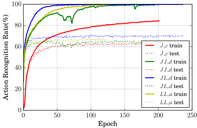
Fig. 16. Performance of four features in the NTU-RGB+D cross-subject setting. Solid and dashed lines represent the training and testing accuracies respectively.
