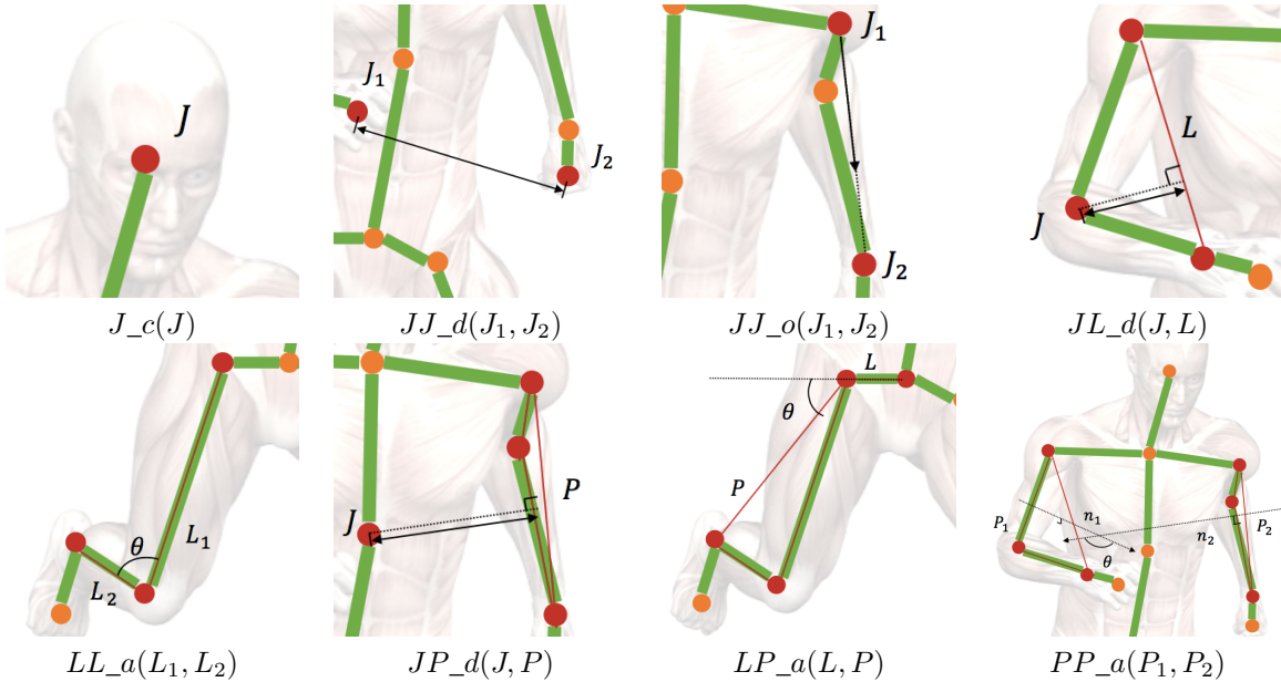
Fig. 5. Eight feature types. Note that for each feature only the relevant joints, lines, and planes are drawn in red.
