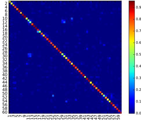
Fig. 9. The confusion matrix of JL_d in the NTU-RGB+D cross-subject setting.
