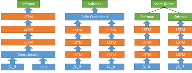
Fig. 6. The illustration of three exploration fusion methods. The input fusion concatenates two features before feeding to network. The fully-connected fusion utilizes a fully-connected layer to combine the two outputs of last LSTM layers. The average fusion computes the average scores of all streams and selects the label with the highest score as prediction.
