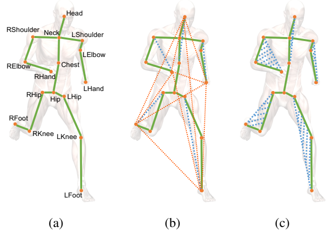
Fig. 4. (a) A skeleton model. Orange dots represent joints and green lines represent limbs. (b) Lines. 15 Green, 5 blue and 10 red lines are three types of lines. (c) Planes.
