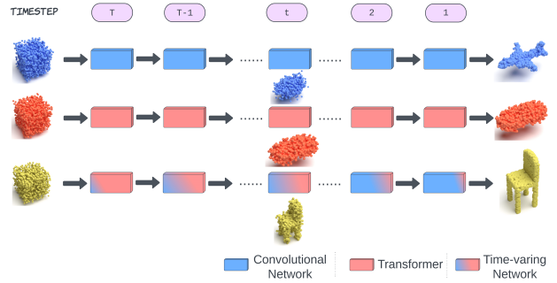
Figure 1. An illustration of different roles played by convolution and attention operations in the denoising model. Convolution is good for learning local relationships, and attention is optimal for modeling global relationships. We propose to merge these two properties across different timesteps in the diffusion process.
